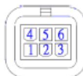
L1-type minifit plug
