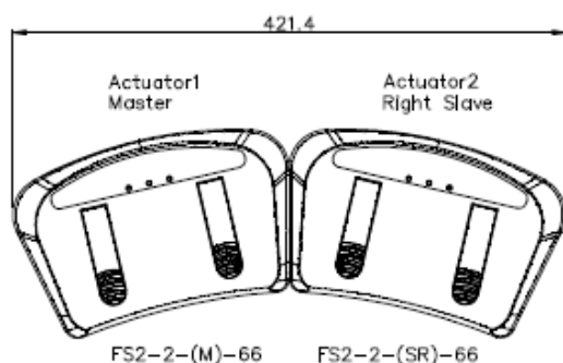
FS2-2-66 Drive2 Actuator
