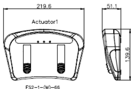
FS2-1-66 Drive1 Actuator
